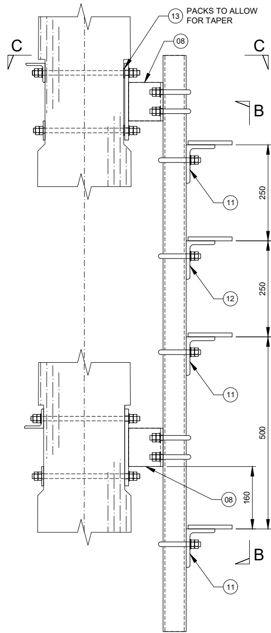
DETAIL H - Tx ANTENNA MOUNT Scale 1:10
