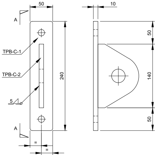
PART TPB-C Scale 1:5 VIEW A-A Scale 1:5
