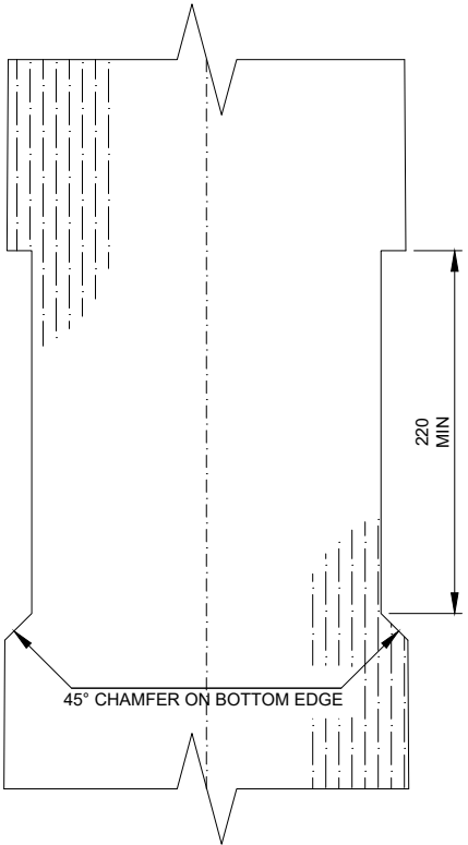
VIEW B-B Scale 1:5
