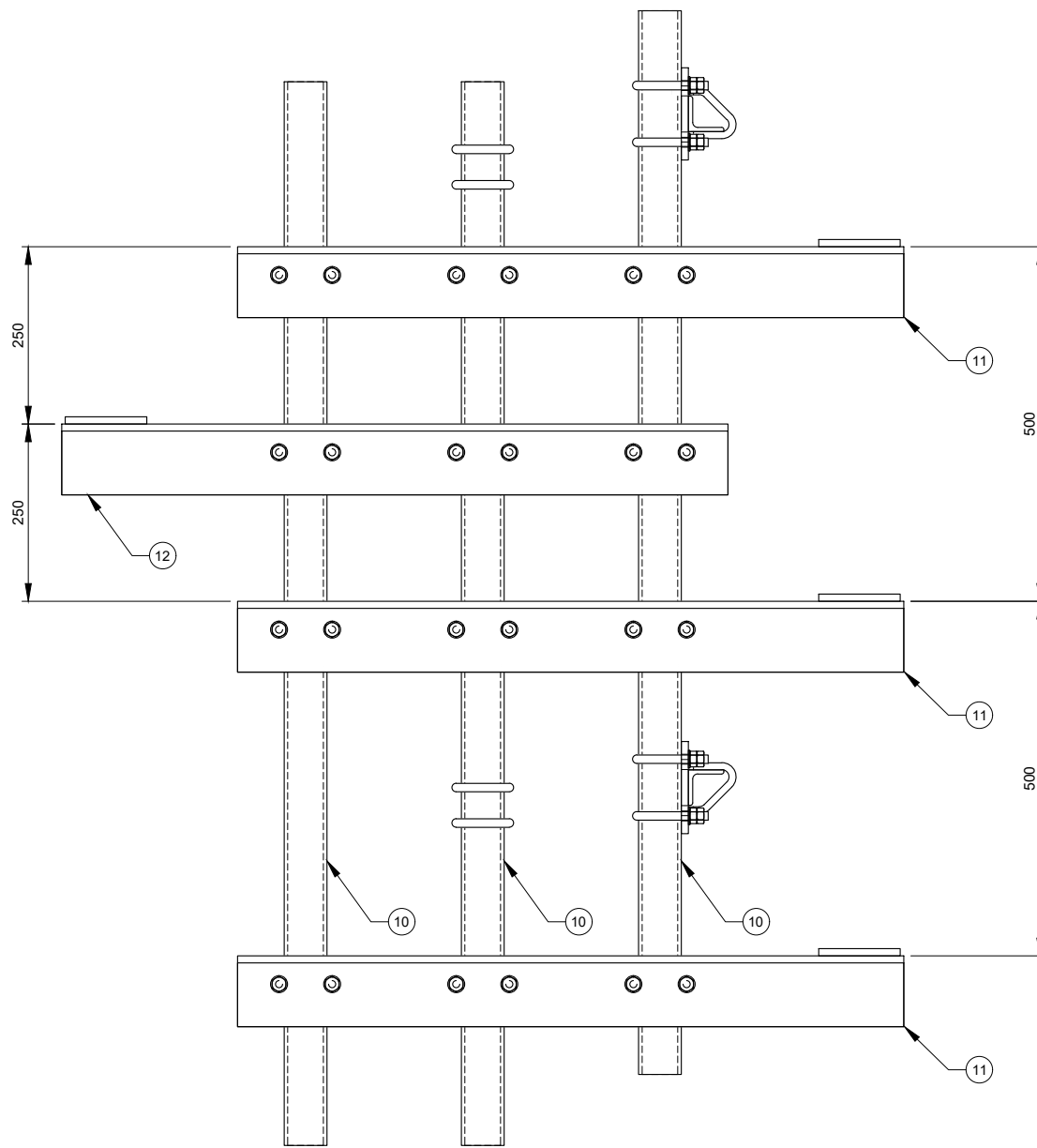
VIEW B-B Scale 1:10
