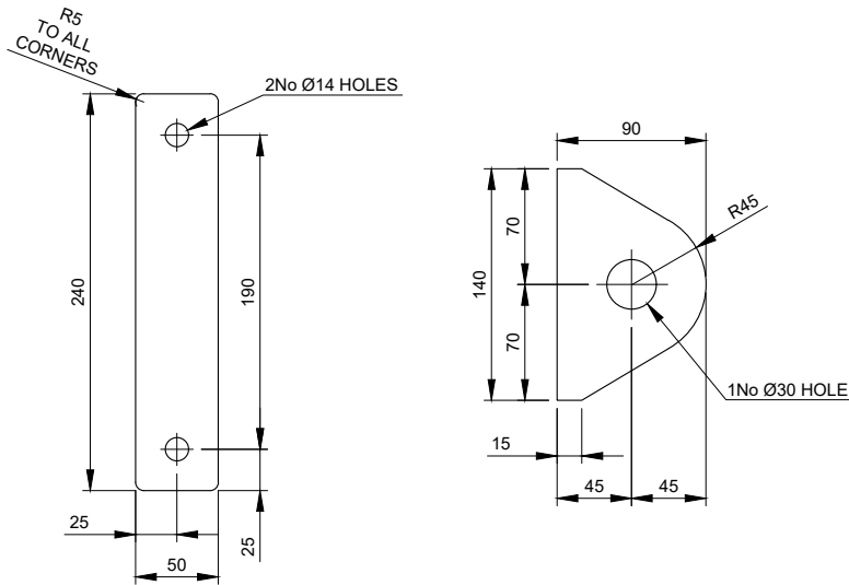
TPB-C-1 - 10mm THICK Scale 1:5 TPB-C-2 - 10mm THICK Scale 1:5
