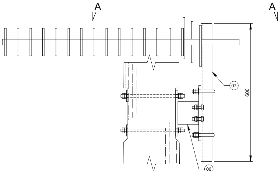
DETAIL G - Rx ANTENNA MOUNT Scale 1:10
