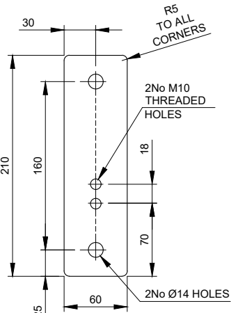
PART TPS-R Scale 1:5
