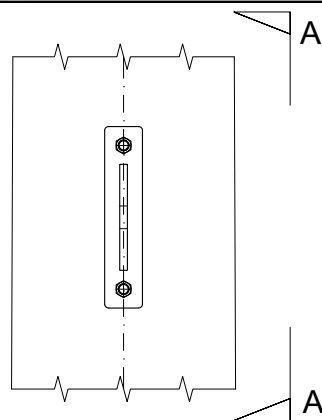
DETAIL C - FALL ARREST ATTACHMENT POINT Scale 1:10
